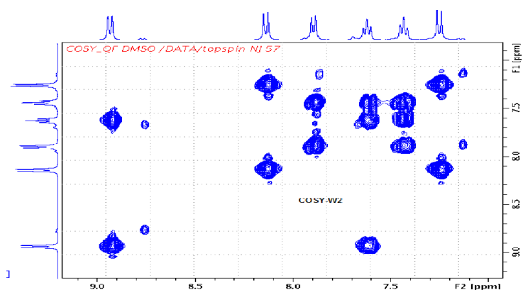
Fig. 5. COSY NMR spectra of cobalt complex compound
