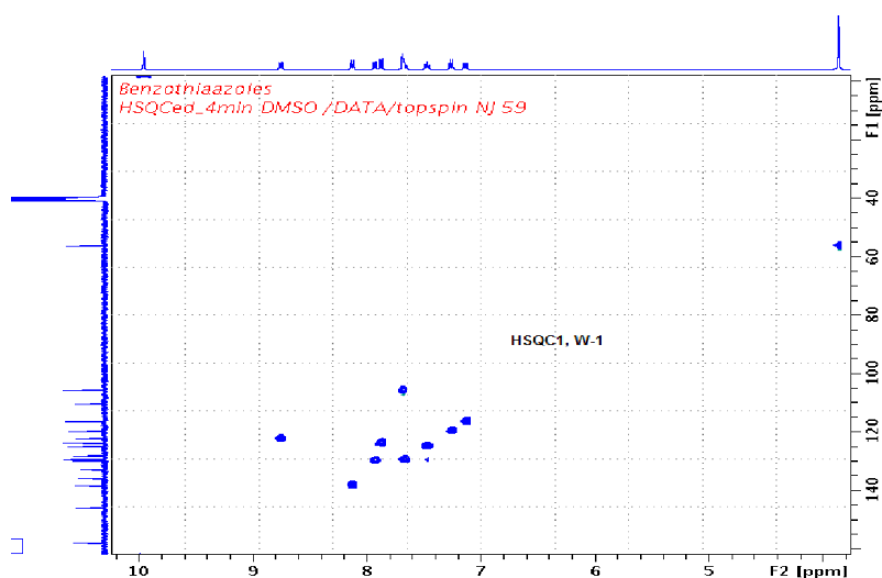
Fig. 3. HSQC NMR spectra of Schiff-base of 6-methoxy benzothiazole (L).
