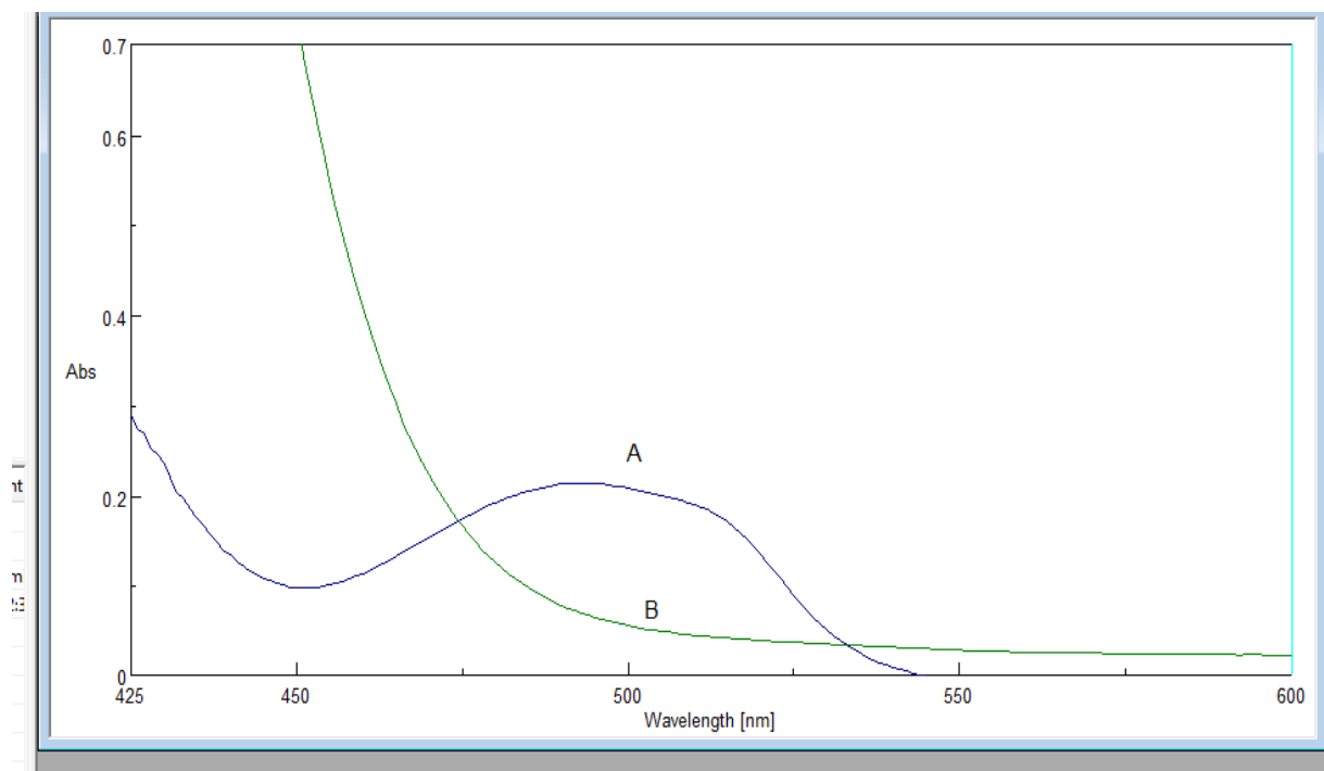
Figure 2: Absorption spectra of 3mg/25ml of mebendazole with 1-fluoro 2, 4-dinitrobenzene against reagent blank(A). Reagent blank against water (B).
